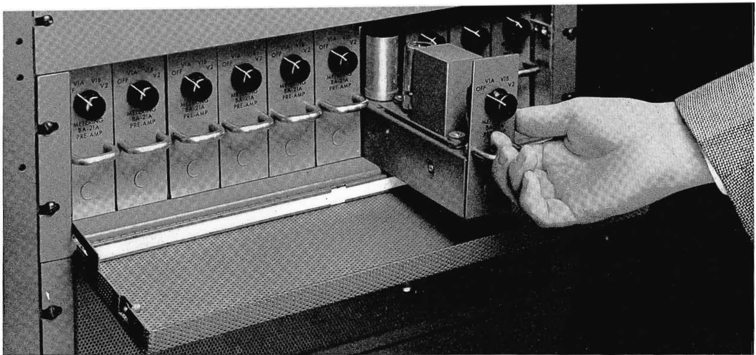
FIG. 2. Photo showing the advantage of space conservation when using miniaturized preamplifiers. Here 10 BA-21A Preamplifiers are accommodated on one shelf.
