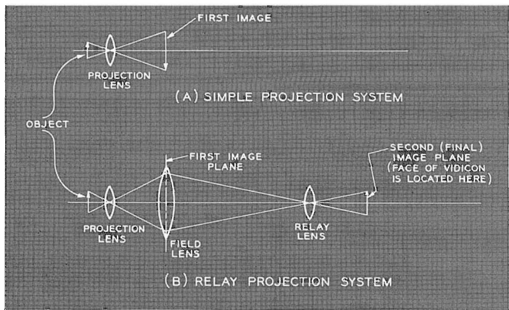
FIG. 5. Comparison of simple projection and relay projection optical system.
