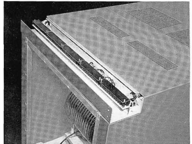
FIG. 7. Detail of completely-shielded interconnection wire duct (cover removed).
