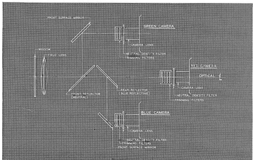
FIG. 6. Optical system of 3-V Color Film Camera.
