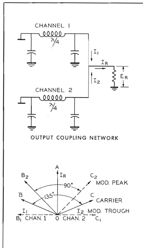
FIG. 3. Vectorial representation of phase-to-amplitude modulation process.
