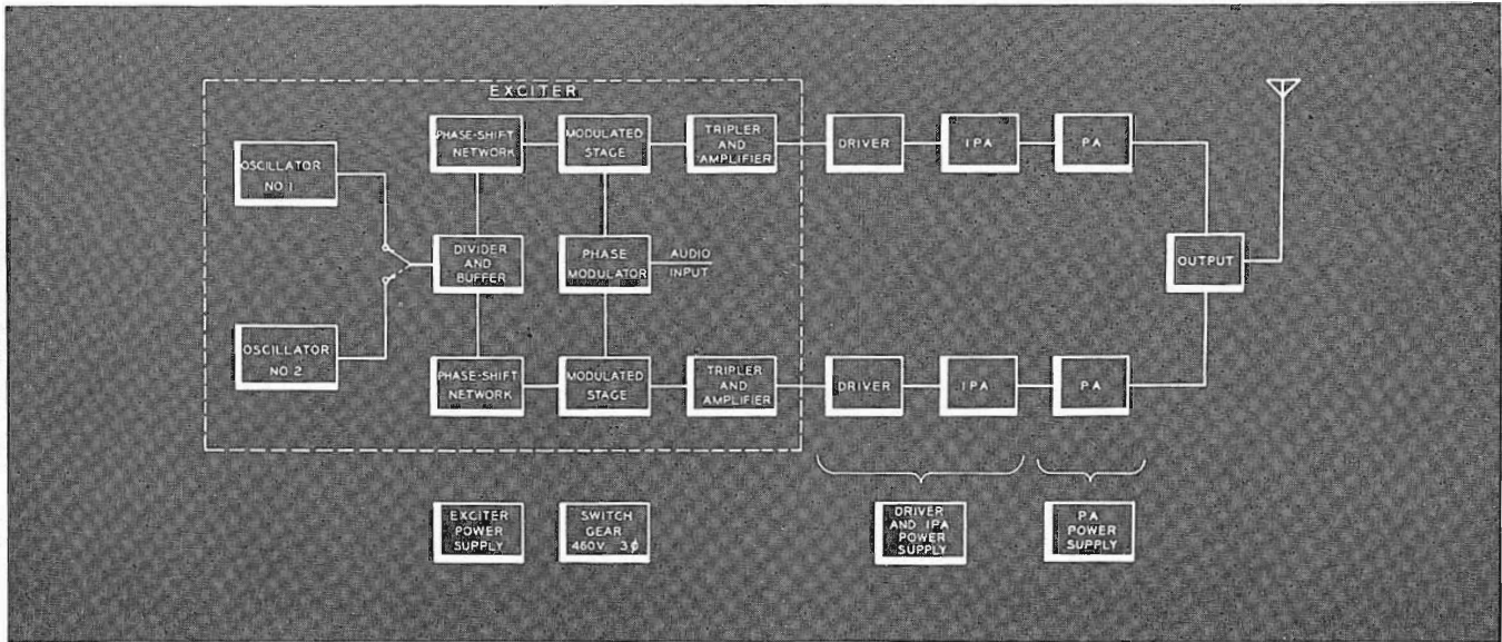
FIG. 2. Simplified Block Diagram of BTA-50G Ampliphase Transmitter.
