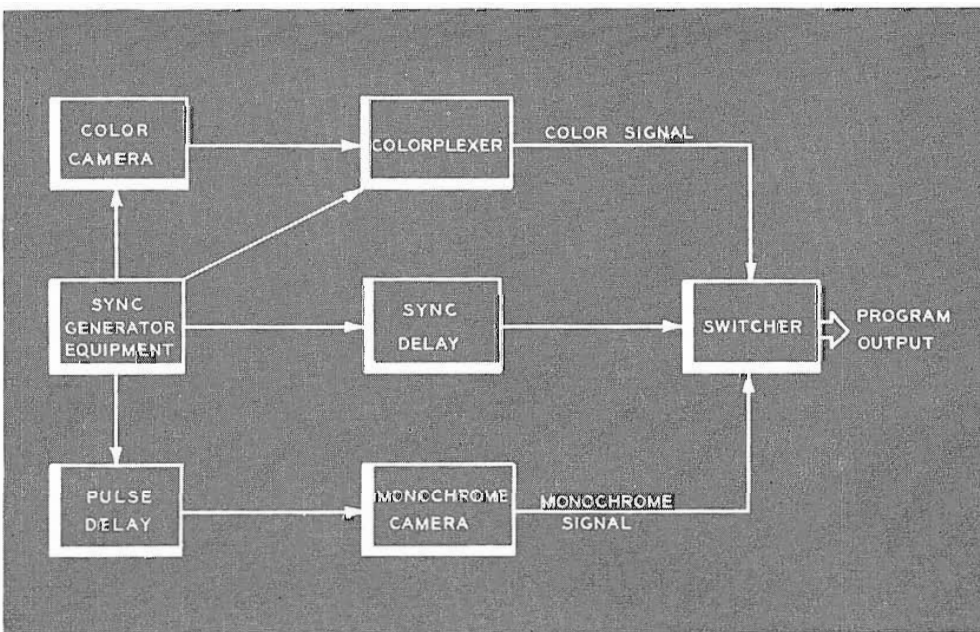
FIG. 2. Delay equalization in color-monochrome system.
