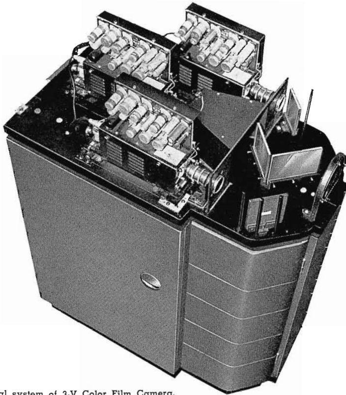
FIG. 4. Optical system of 3-V Color Film Camera.
