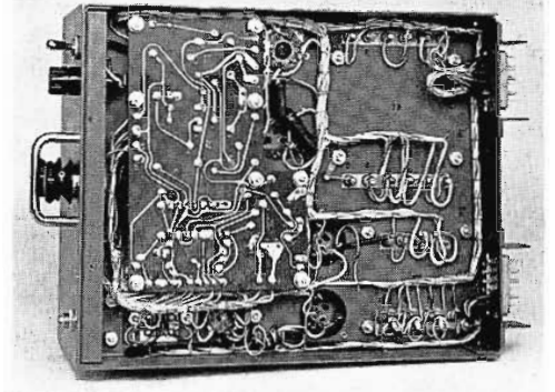
FIG. 8. Underside of a BA-24A Monitoring Amplifier. Note etched-wiring circuit board on left.
