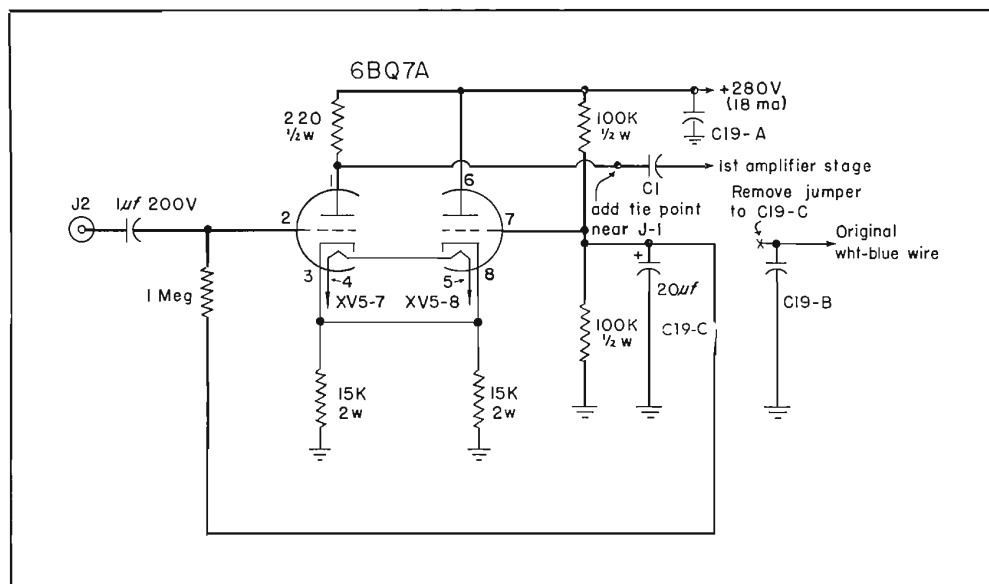
FIG. 6. Schematic of Polarity Inversion Modification for TA-3A Distribution Amplifier.
