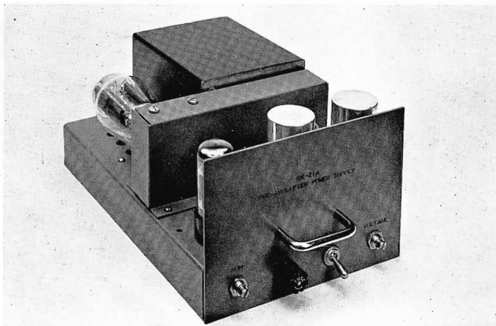
FIG. 3. A compact power supply (BX-21A) furnishes power for ten BA-21A Preamplifiers.
