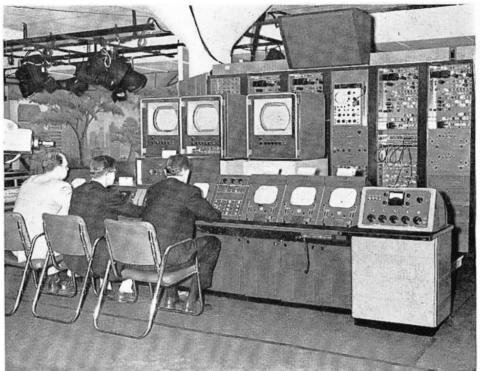
TELEVISION CONTROL CENTER . . . Control and rack equipments for all operating displays in the exhibit were located in this area. Color monitors (l. to r.) showed pictures from live color camera, 3-V color film camera, and color effects equipment. New masking amplifier for 3-V equipment is shown in front of the center monitor. Remote control panel for TP-15 Multiplexer is mounted in remote control housing (center).
