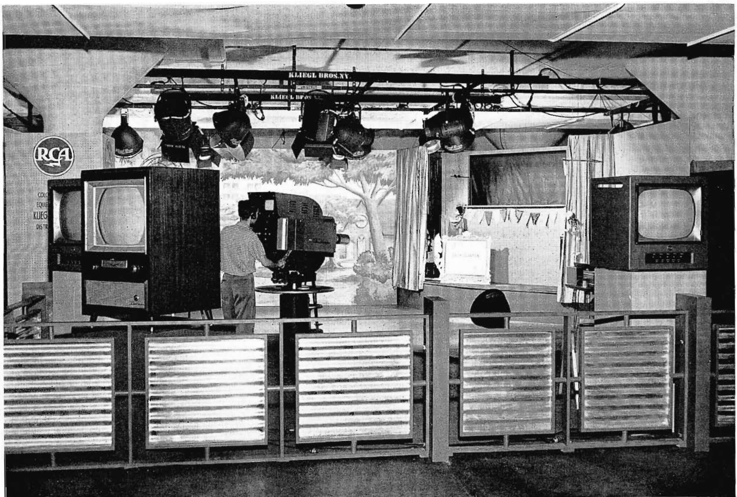
OVERALL VIEW OF LIVE COLOR STUDIO . . . The color studio occupied 900 square feet. Two separate sets, a puppet stage and a park scene occupied this area. Studio pictures were seen on two 21 inch RCA Color TV receivers and on two 21 inch black-and-white utility monitors. The RCA TK-41 Live Color Camera operated throughout the exhibit hours.
