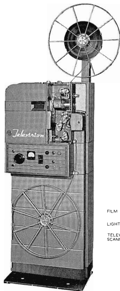
◀ FIG. 22. TP-6BC 16mm TV Motion Picture Projector.
