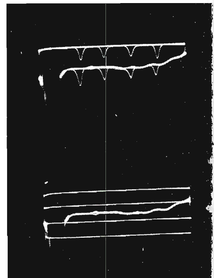
FIG. 7. Envelope delay of BW-4 Demodulator with frequency markers at 1, 2, 3 and 4 mc (top); delay markers spaced at 0.1 \mu sec (bottom).
