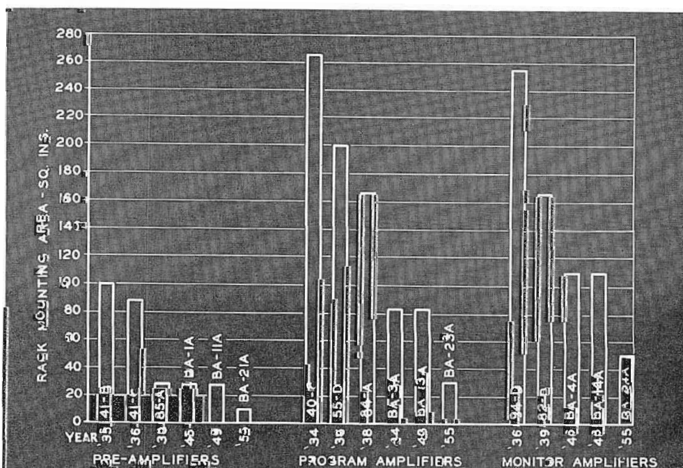
FIG. 11. Chart showing yearly progress in amplifier space conservation.
