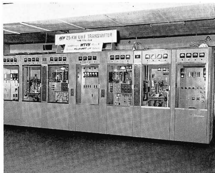
NEW 25 KW UHF TRANSMITTER, TTU-25B . . . Shown for the first time, this transmitter plus an RCA Ultra-Gain Pylon Antenna will enable UHF Broadcasters to obtain 1,000,000 watts ERP. Transmitter shown occupies the same floor space as the RCA 12½ KW UHF Transmitter. Owners of RCA 12½ KW's can obtain conversion parts so they too may go to maximum power.
