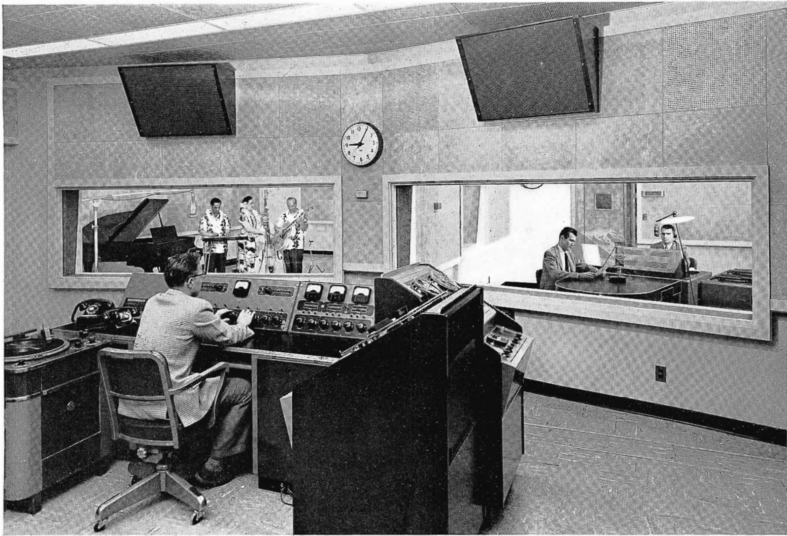
FIG. 14. AM Master Control Room in new WHIO Studio Building. The three AM studios are grouped about this control room so that there is direct visual communication between all three and the control room. An RCA BC-2B Console and RCA BCS-11A Switcher provide flexible facilities with a high degree of operating efficiency.
