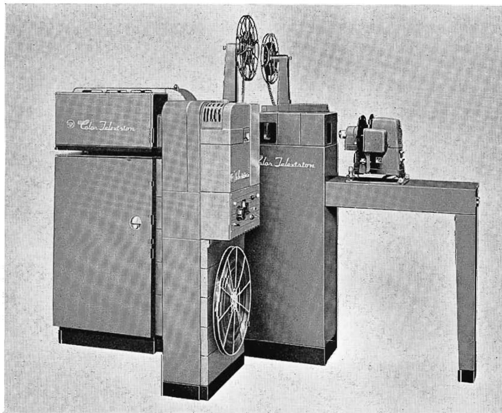
FIG. 20. Complete 3-V film system employing TP-12 multiplexer.
