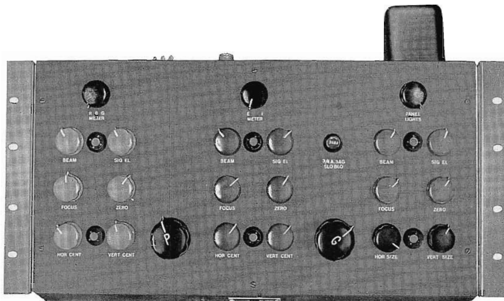
FIG. 12. Camera control panel.
