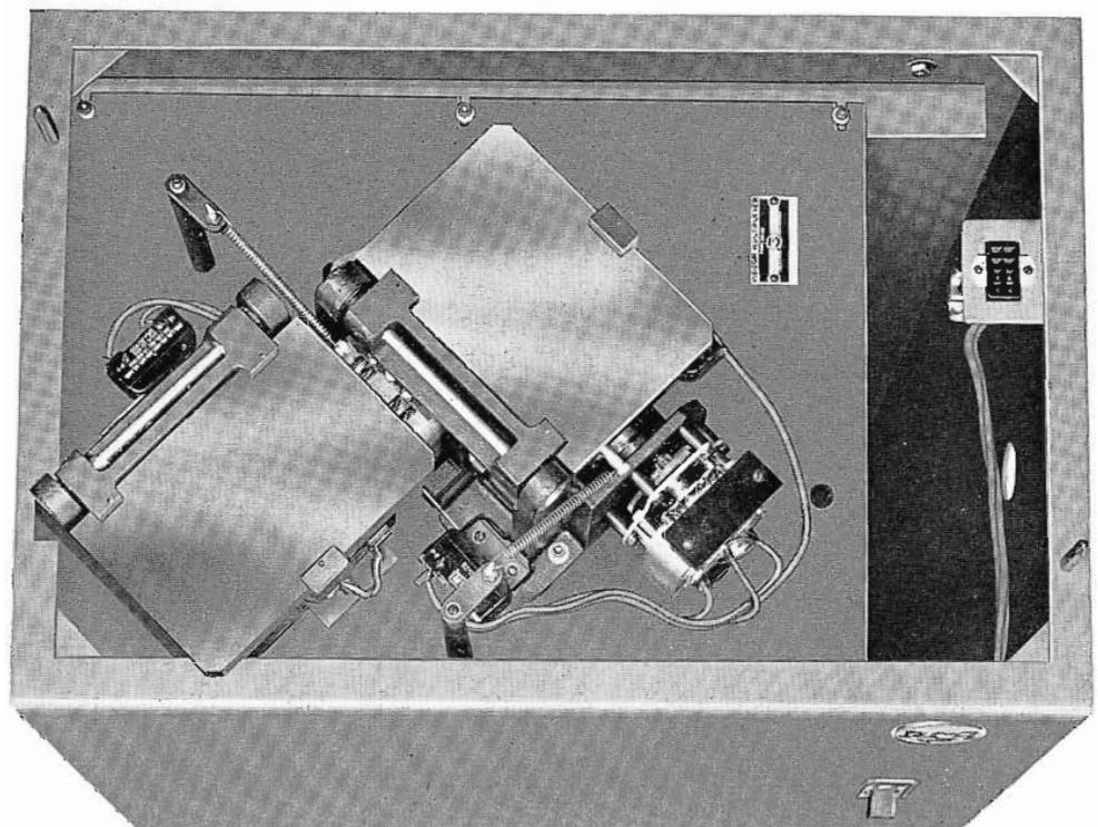
FIG. 28. Mirror arrangement of TP-12 multiplexer showing Geneva mechanism used to rotate front-surfaced mirrors (top view).
