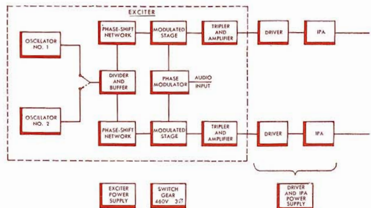
SIMPLIFIED BLOCK DIAGRAM—BTA-50G TRANSMITTER
