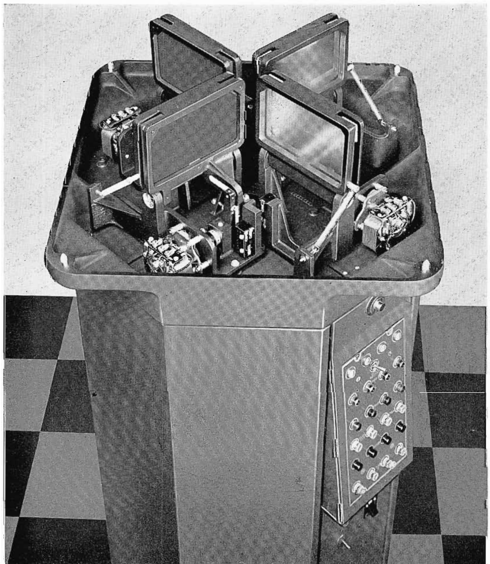
FIG. 9. Mirror star of the 3-V Multiplexer. Local control panel is visible in the lower right corner.
