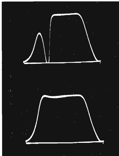
FIG. 5. IF response of BW-4 Demodulator as shown on the oscilloscope with sound notch-in (top); sound notch-out (bottom).
