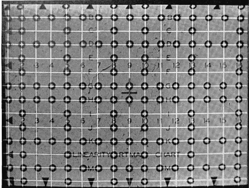
FIG. 14. Performance of system shows that linearity is better than 1 per cent in both directions.
